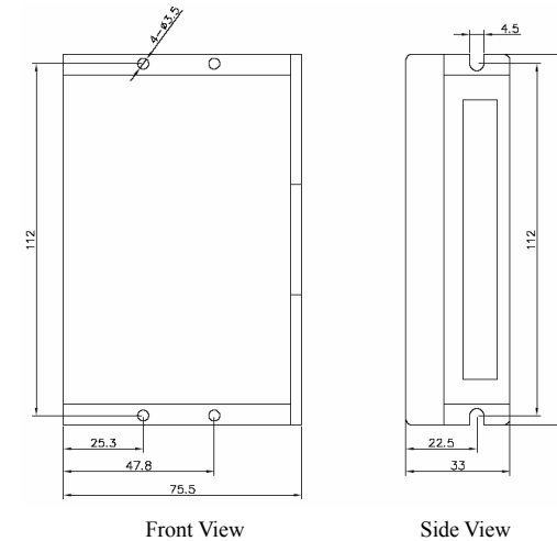
Figure 1: Mechanical dimensions
