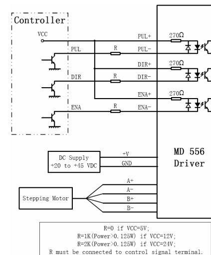
Figure 9: Typical connection
