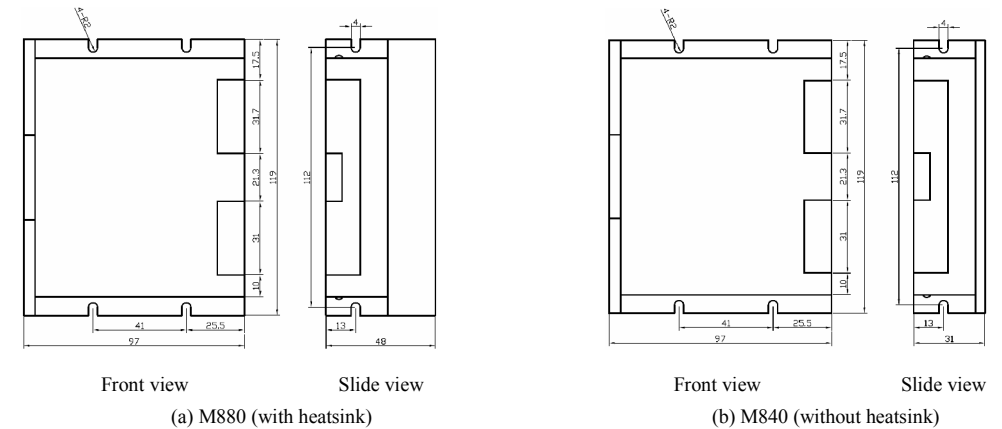
Figure 1: Mechanical specifications
