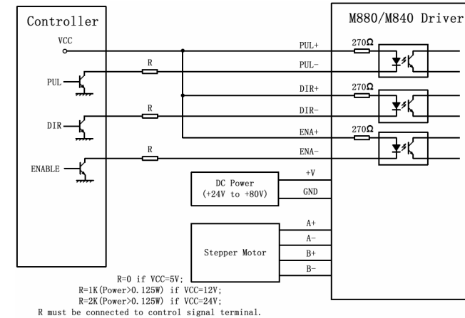
Figure 10: Typical connection
